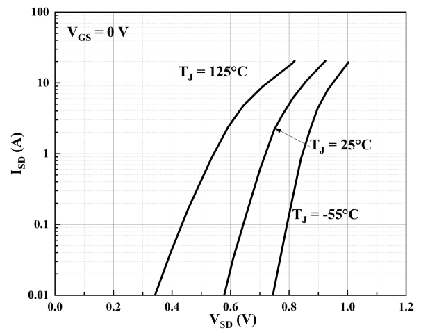
Figure 4. Body-Diode Characteristics
