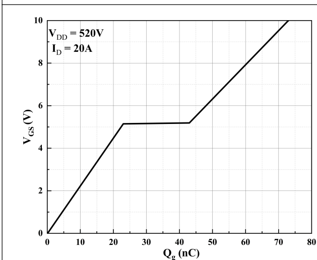
Figure 5. Gate-Charge Characteristics
